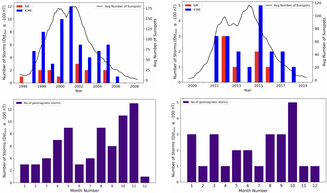
Figure 2. Top panel: The bar plots show number of geomagnetic storms with Dst_{\min} \leq -100 nT, for each year from 1996 to 2008 in solar cycle 23 in the left and from 2009 to 2019 for solar cycle 24 in the right. The blue and red bars represent the storm’s drivers as ICME and SIR, respectively. Bottom panel: Monthly distribution of the total number of storms for solar cycles 23 and 24 in the left and right panels, respectively.
